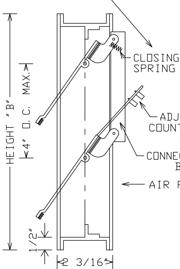
VERTICAL SECTION
