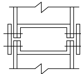
HORIZONTAL MULLION (VERTICAL SIMILAR)
