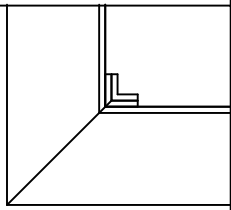
MITER CORNER DETAIL
