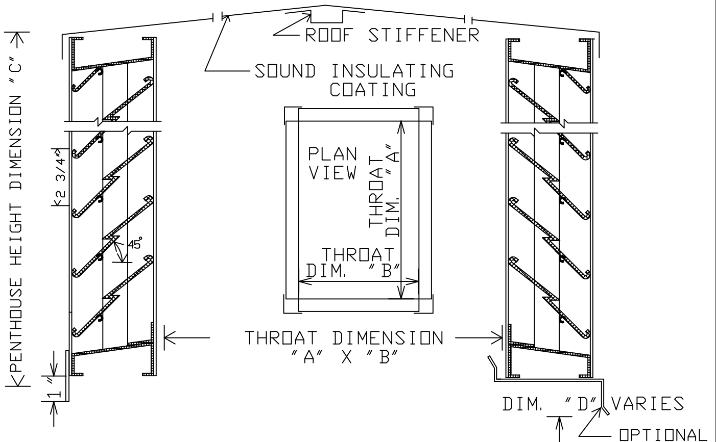
VERTICAL SECTION
