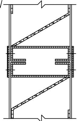
HORIZONTAL MULLION
