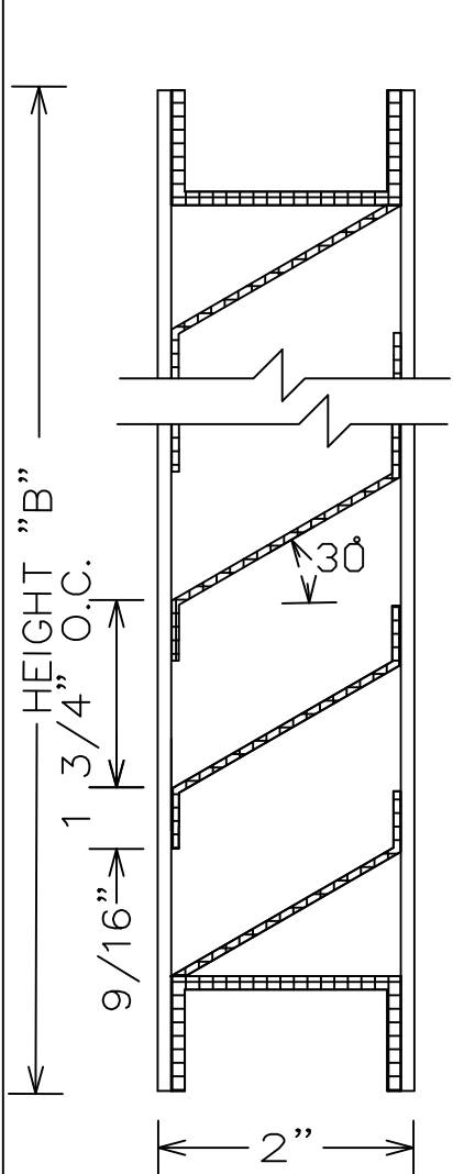
VERTICAL SECTION
