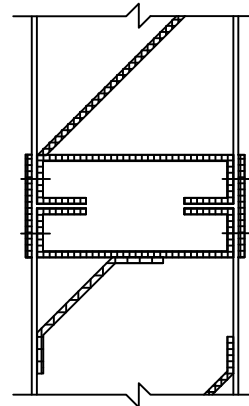
HORIZONTAL MULLION
