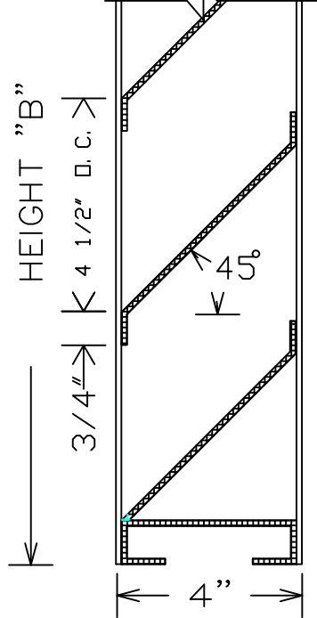
VERTICAL SECTION
