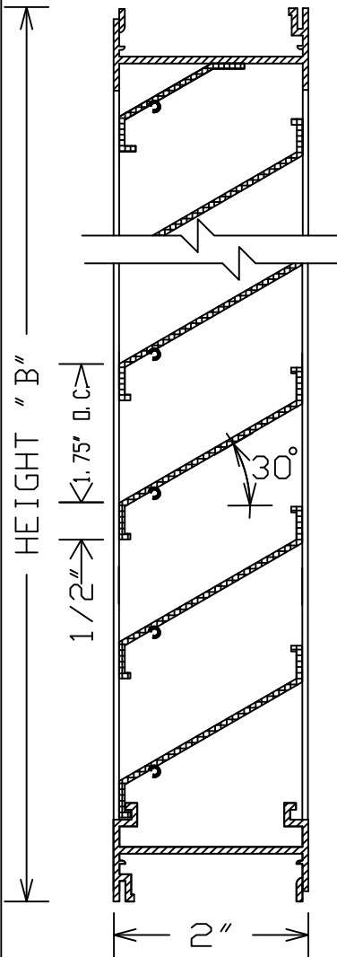
VERTICAL SECTION
