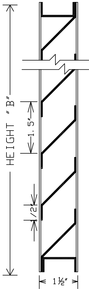
VERTICAL SECTION STANDARD TL-45
