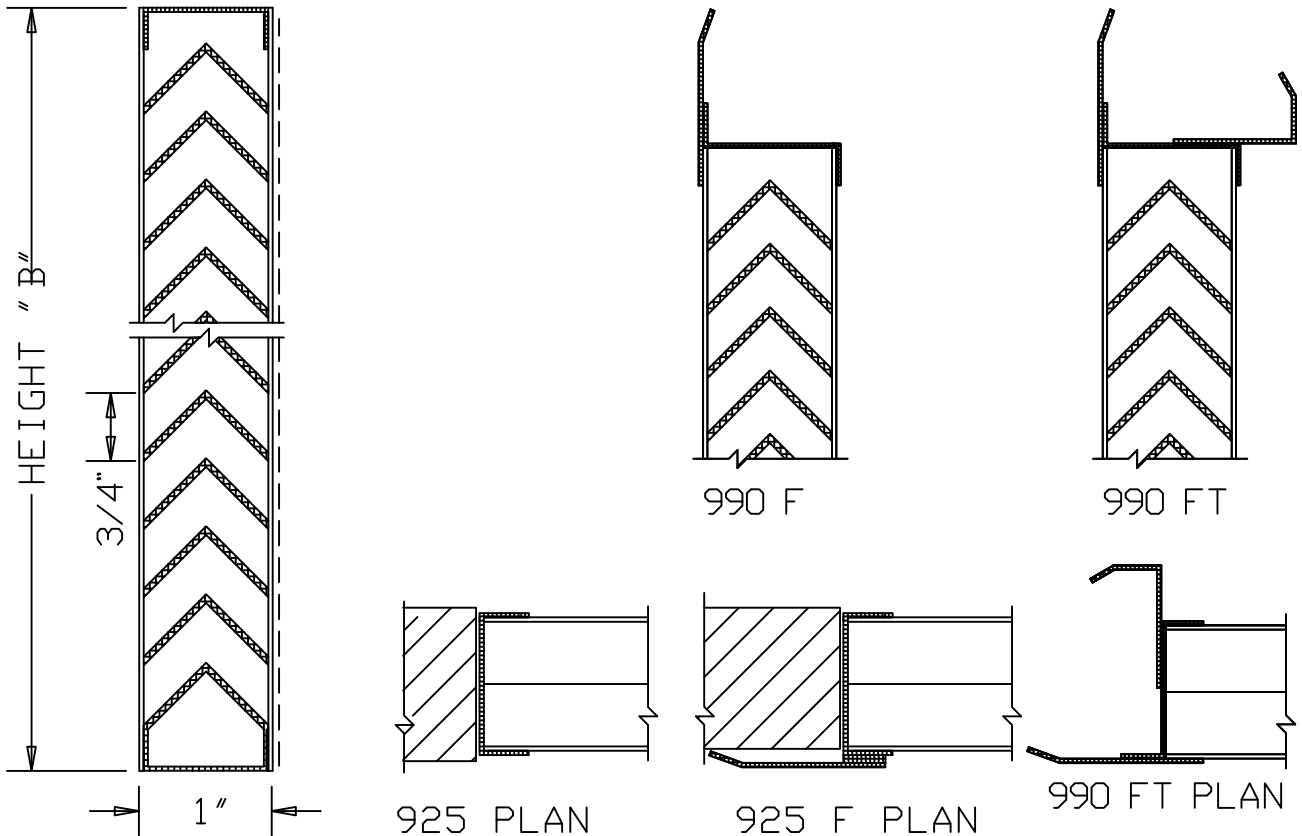
VERTICAL SECTION
