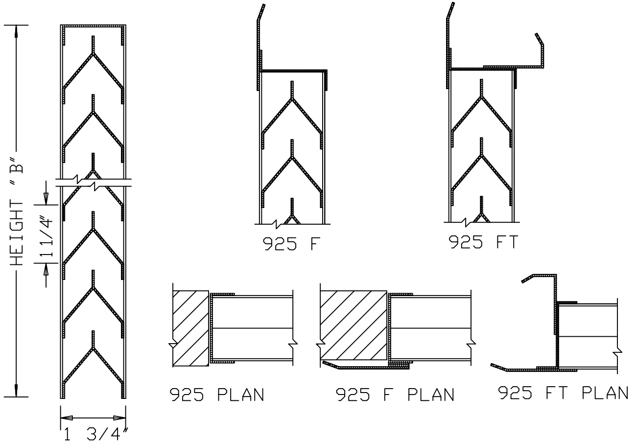
VERTICAL SECTION STANDARD 925
