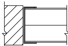
922 PLAN
