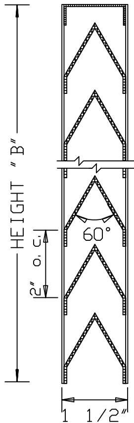
VERTICAL SECTION STANDARD 922
