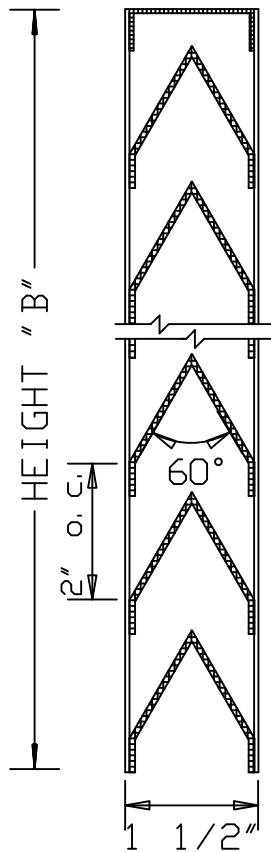
VERTICAL SECTION
