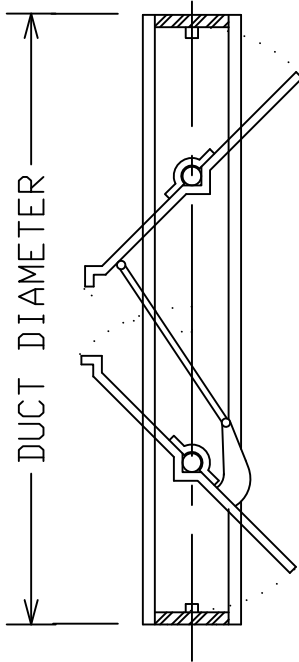
VERTICAL SECTION (OPEN)
