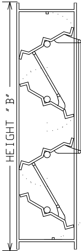
VERTICAL SECTION
