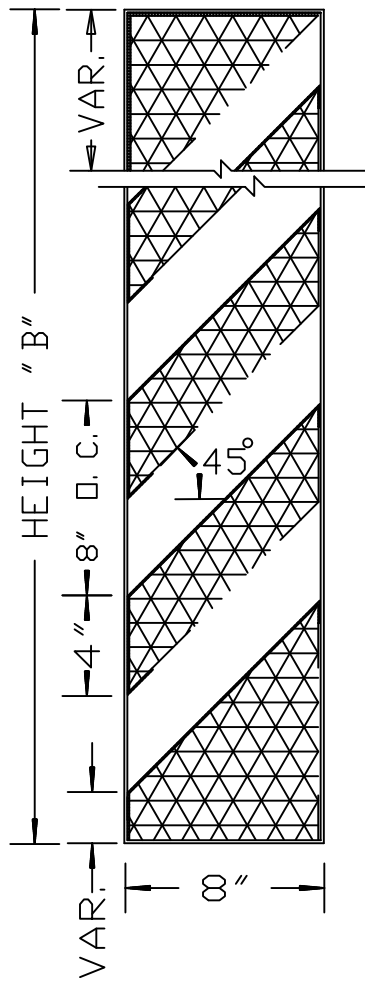
VERTICAL SECTION
